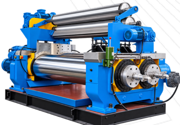
Rubber Mixing Mill
